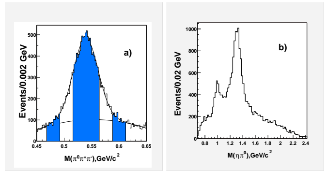
FIG. 1: (a) Fit of the \pi^+ \pi^- \pi^0 mass distribution in the \eta mass region. There are two entries per event: one for each way to assign a \pi^0 to the \eta decay. The \eta signal region and the side-band regions are shown shaded. (b) The uncorrected \eta \pi^0 effective-mass distribution for events consistent with the reaction \pi^- p \rightarrow \eta \pi^0 n
