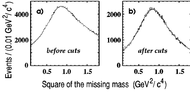
FIG. 2. Experimental distribution of the square of the missing mass: (a) Without cuts on soft \pi^0 's and azimuthal angle between recoil track and missing momentum; (b) after the cuts. The curve represents a fit with a Gaussian function centered at the square of the proton mass with \sigma=0.260 ( \text{GeV}/c^2 ) 2 .
